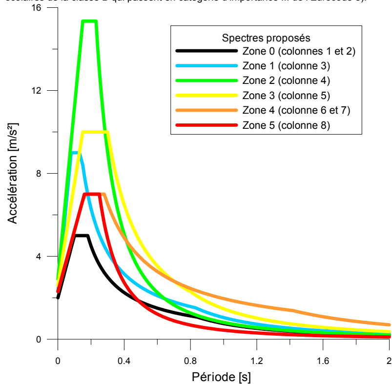
Figure 8 - Spectres des 6 zones du microzonage
